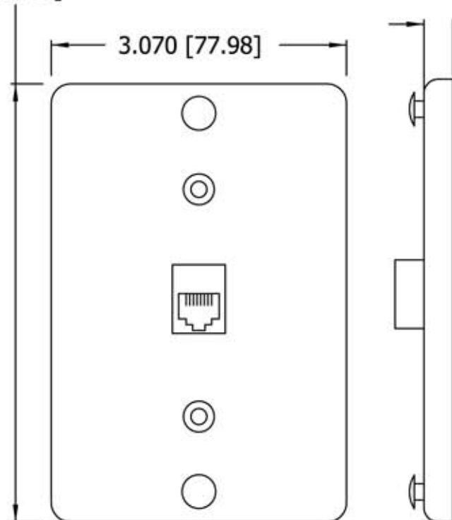
STAINLESS STEEL COVER
